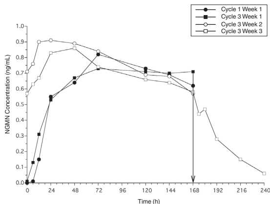
Figure 1: Mean Serum NGMN Concentrations (ng/mL) in Healthy Female Volunteers Following Application of ORTHO EVRA® on the Buttock for Three Consecutive Cycles (Vertical arrow indicates time of patch removal)
