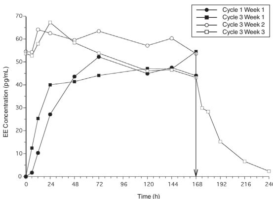
Figure 2: Mean Serum EE Concentrations (pg/mL) in Healthy Female Volunteers Following Application of ORTHO EVRA® on the Buttock for Three Consecutive Cycles (Vertical arrow indicates time of patch removal.)
