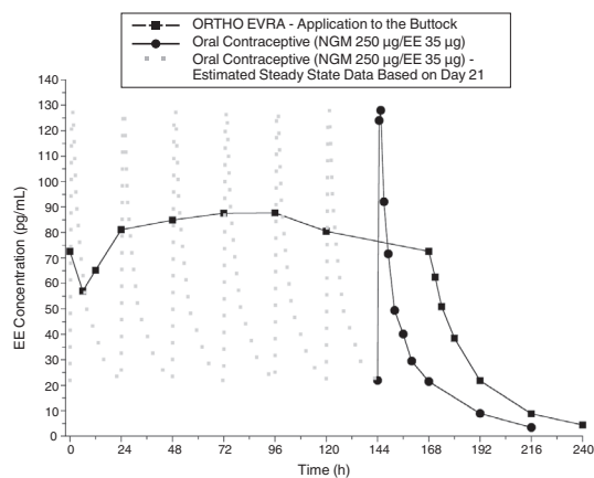
Figure 4: Mean Serum Concentration-Time Profiles of EE Following Once-Daily Administration of an Oral Contraceptive for 2 Cycles or Application of ORTHO EVRA® for 2 Cycles to the Buttock in Healthy Female Volunteers. [Oral contraceptive: Cycle 2, Days 15-21, ORTHO EVRA®: Cycle 2, Week 3]
